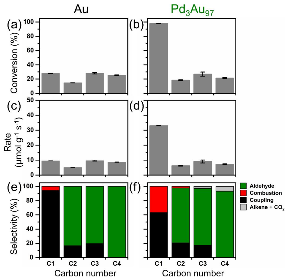
Figure 2. The conversion of C1 to C4 alcohols and the rate of alcohol oxidation at 423 K over (a,c) Au and (b,d) Pd 3 Au 97 RCT-SiO 2 , and the corresponding selectivity over (e) Au and (f) Pd 3 Au 97 RCT-SiO 2 . Reaction products in (e,f) are listed in Table S4. Complete data sets are listed in Table S5. Reaction conditions: 4% alcohol, 10% O 2 , balanced in He; total flow rate = 50 mL/min; m cat = 40.0 and 40.5 mg for Au RCT-SiO 2 and Pd 3 Au 97 RCT-SiO 2 , respectively.
