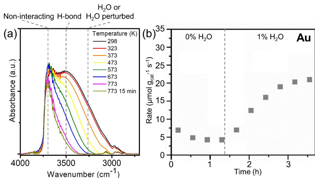
Figure 1. (a) In-situ FTIR spectra of as-prepared Au RCT-SiO 2 in the 4000-2700 cm -1 region collected as a function of temperature from 298 to 773 K in O 2 . (b) The rate of 1-propanol oxidation over Au RCT-SiO 2 in the absence and presence of co-fed 1% H 2 O at 423 K. Dashed lines in (a) denoted the assignments of silanol groups. Reaction conditions in (a): 100% O 2 ; flow rate = 20 mL/min, (b): 4% 1-propanol, 10% O 2 , 0 or 1% H 2 O, balanced in He; total flow rate = 50 mL/min; m cat = 10.0 mg.
