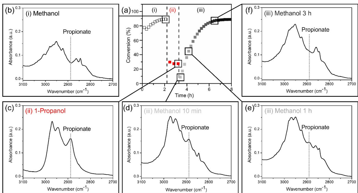
Figure 5. (a) The conversion of (i) methanol oxidation for 2 h, (ii) 1-propanol oxidation for 1 h after replacing methanol with 1-propanol, and (iii) re-establish methanol oxidation for 5 h after replacing 1-propanol with methanol at 423 K over Pd 3 Au 97 RCT-SiO 2 . (b-f) The corresponding in-situ FTIR spectra in the 3100-2700 cm -1 region representing different stages of the experiment, including during (b) (i) methanol oxidation, (c) (ii) 1-propanol oxidation, and (d-f) (iii) re-establishing methanol oxidation after replacing 1-propanol with methanol. Dashed lines in (a) indicated the replacement of reactants, and in (c-f) denoted the IR peak of interest. Reaction conditions: 4% alcohol and 10% O 2 balanced in He; total flow rate = (a) 50 and (b) 20 mL/min; m cat in (a) = 40.5 mg.
