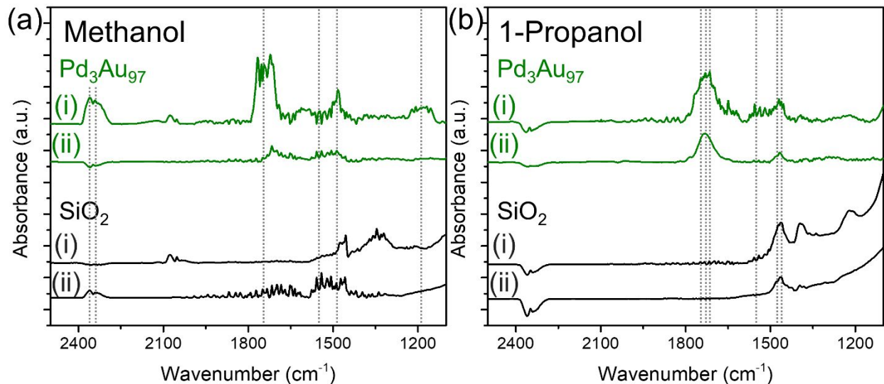
Figure 4. In-situ FTIR spectra in the 2500-1100 cm -1 region collected (i) during the oxidation of (a) methanol and (b) 1-propanol over Pd 3 Au 97 RCT-SiO 2 (green) and RCT-SiO 2 (black) at 423 K for 1.5 h and followed by (ii) purging in He for 2 h. Reaction conditions: 4% alcohol and 10% O 2 , balanced in He; total flow rate = 20 mL/min. Dashed lines denoted the peaks of interest with peak assignments summarized in Table 2.
