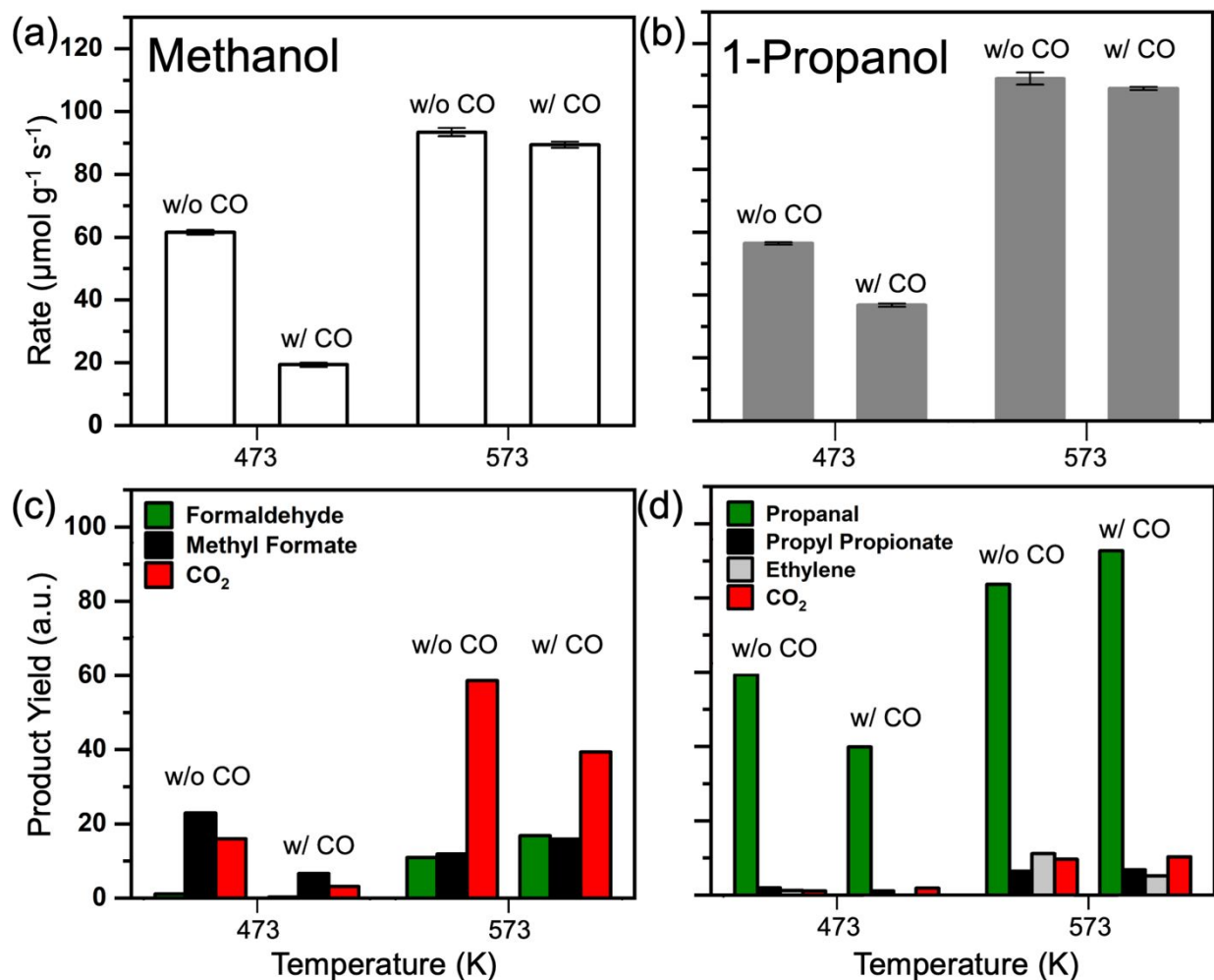
Figure 3. The rate of (a) methanol and (b) 1-propanol oxidation in the absence (w/o CO) and presence (w/ CO) of co-fed 2% CO at 473 K and 573 K over Pd 3 Au 97 RCT-SiO 2 , and the corresponding yield of products during (c) methanol and (d) 1-propanol oxidation. Reaction conditions: 4% 1-propanol, 10% O 2 , 0 or 2% CO, balanced in He; total flow rate = 50 mL/min; m cat = 10.0 mg.
