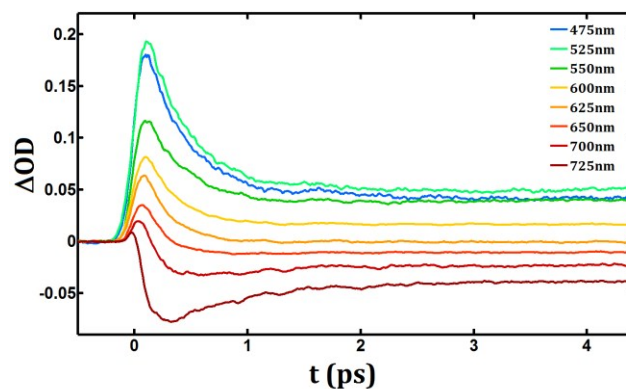
Fig. 3. Change of optical density at different probe wavelengths after fs excitation at 850 nm measured on [Fe III (3-MeO-SalEen) 2 ]PF 6 nano-crystals. Measurements are performed at 100K in pure LS state.
