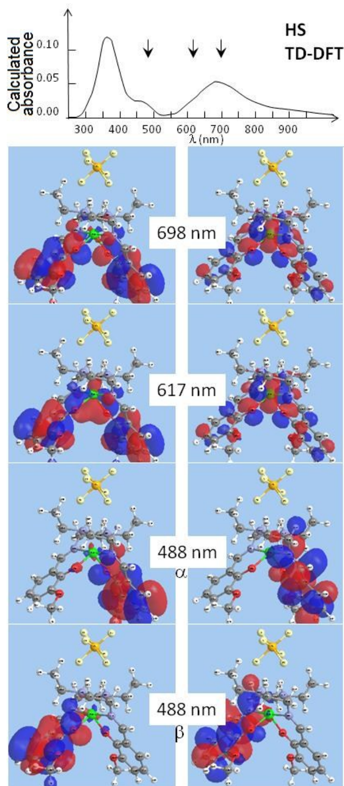
Fig. 9. Natural transition orbitals of hole (left) and particle (right) calculated in the case of HS species at 698, 617 and 488 nm, i.e. close to the experimental probes at 700, 625 and 550–475 nm. \alpha and \beta designate spin \uparrow and spin \downarrow . The calculated absorbance spectrum (top) underline the strong weight of these transitions.
