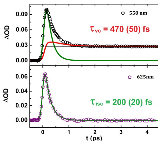
Fig. 4. Deconvolution of raw data into the relaxation kinetic of the INT electronic states ( \tau_{isc} , green line) and the population kinetic of the HS state taking into account vibrational cooling ( \tau_{vc} , red line). Only 1/8 of the experimental data are shown for clarity.
