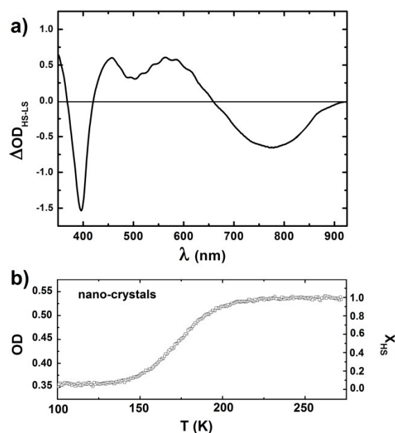
Fig. 1 Difference of optical density in the (350-925 nm) spectral window between HS state (296 K) and LS state (16 K) measured on the nano-crystals sample (a). Photo-excitation is performed at 850 nm in the tail of the LS absorption band. OD at 550 nm (left axis) of the nano-crystal assembly during the crossover scaled to X_{HS} (right axis) (b).
