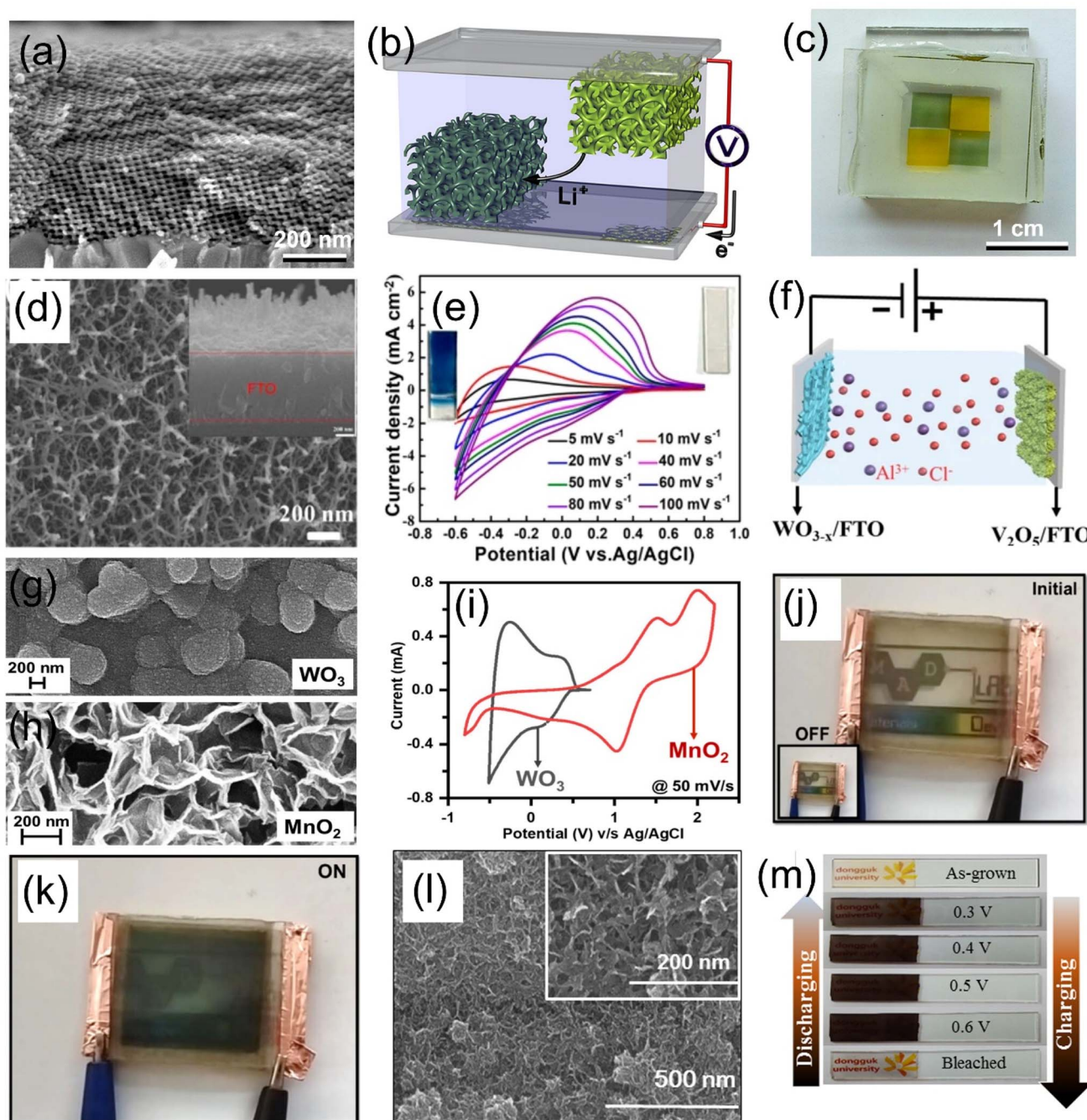
Fig. 12 (a) Cross-sectional SEM image of mesoporous \text{V}_2\text{O}_5 double-gyroid films. (b) Illustration of the SCs based on \text{V}_2\text{O}_5 double-gyroid film electrodes. (c) Photograph of transparent electrochromic SCs. 112 Reproduced with permission. 112 Copyright 2012, American Chemical Society. (d) SEM image of the \text{WO}_{3-x} NWNs/FTO electrode and its corresponding (e) CV curves at different scan rates. (f) Illustration of the assembly of an electrochromic SC device using the \text{WO}_{3-x} NWNs/FTO anode and \text{V}_2\text{O}_5 nanoflowers/FTO cathode. 113 Reproduced with permission. 113 Copyright 2021, Springer Nature. SEM images of the (g) \text{WO}_3 electrode and (h) \text{MnO}_2 electrode. (i) CV curves of \text{WO}_3 and \text{MnO}_2 electrodes at 50 \text{ mV s}^{-1} . Photographs of the device based on \text{WO}_3 and \text{MnO}_2 electrodes in (j) initial state and (k) ON state. 114 Reproduced with permission. 114 Copyright 2025, American Chemical Society. (l) SEM images of the \text{NiMoO}_4 film. (m) Photograph of the \text{NiMoO}_4 electrode bleached at different voltage potentials. 115 Reproduced with permission. 115 Copyright 2018, Elsevier.
