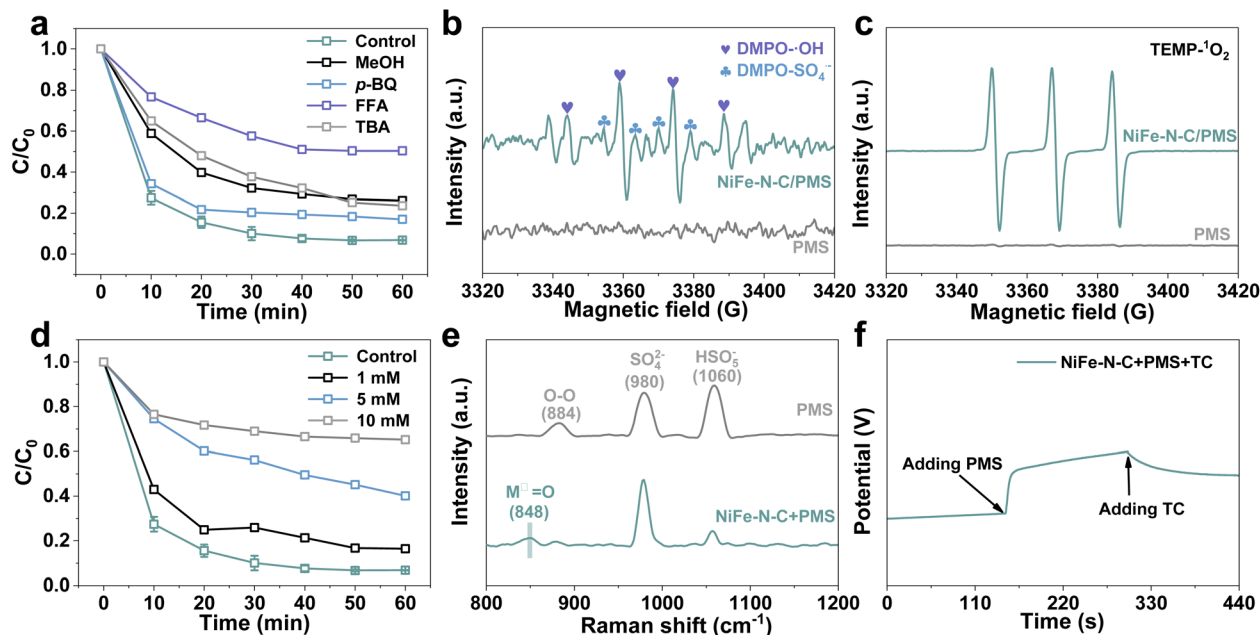
Fig. 4 (a) TC degradation with different kinds of scavengers; EPR spectra of (b) DMPO- \cdot OH and DMPO-SO 4 · - , and (c) TEMP- 1 O 2 ; (d) quenching experiments of the NiFe-N-C/PMS systems by using DMSO; (e) Raman spectra of PMS and NiFe-N-C/PMS systems; (f) open-circuit potential tests.
