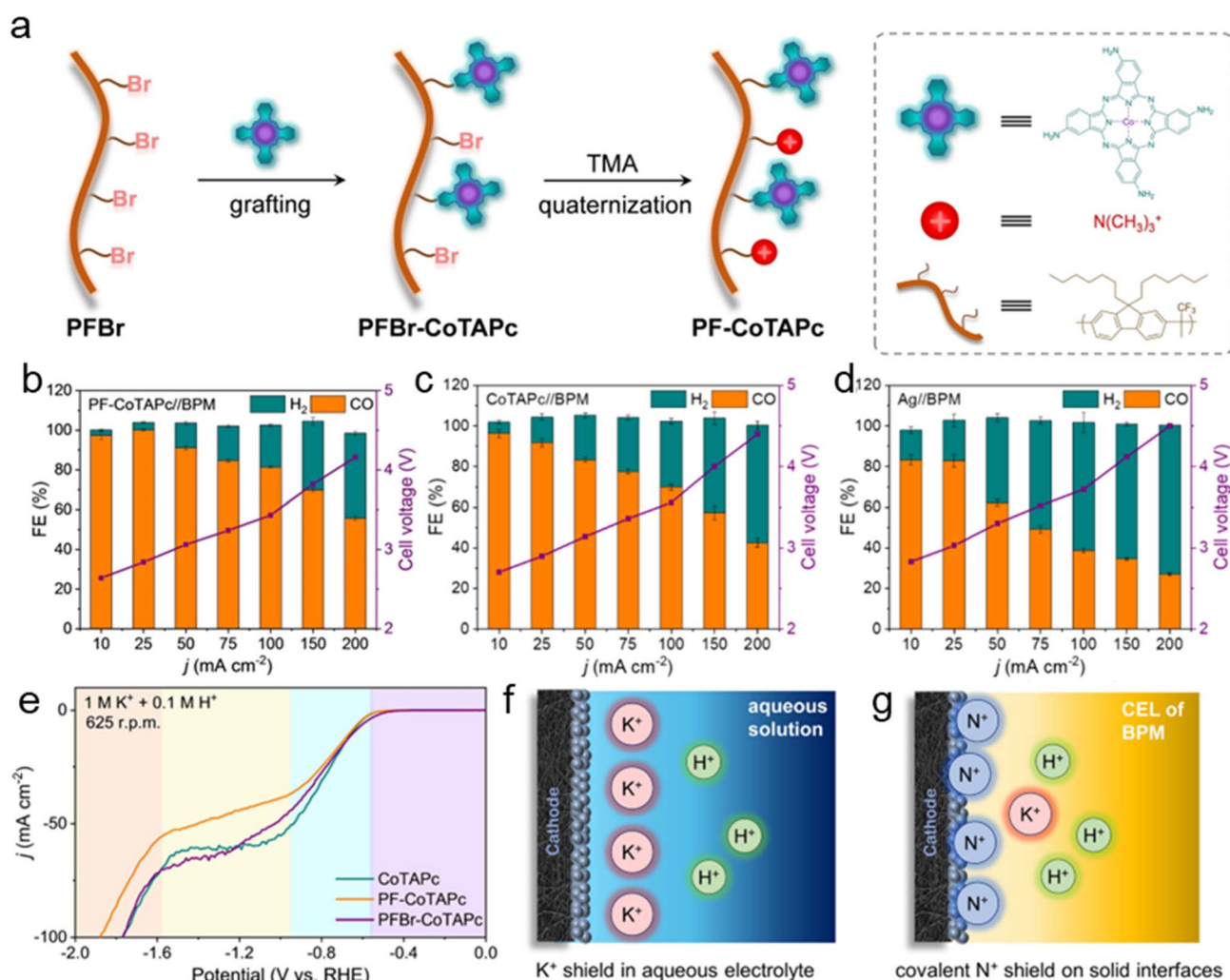
Fig. 8 (a) Synthesis of polymeric catalyst PF-CoTAPc. (b)–(d) \text{CO} , \text{H}_2 FE and cell voltage of PF-CoTAPc (b), CoTAPc (c) and Ag (d) in a BPM-based zero-gap electrolyzer. (e) LSV curves collected at a scan rate of 40\text{ mV s}^{-1} in \text{N}_2 -saturated solutions ( 1\text{ M K}^+ and 0.1\text{ M H}^+ ) at rotating speeds of 625\text{ rpm} . (f) and (g) Illustration of local fields at the diffusion layers for (f) conventional method with high-concentration alkali metals and (g) covalent grafting of quaternary ammonium groups. Reproduced with permission. 141 Copyright 2024 Wiley.
