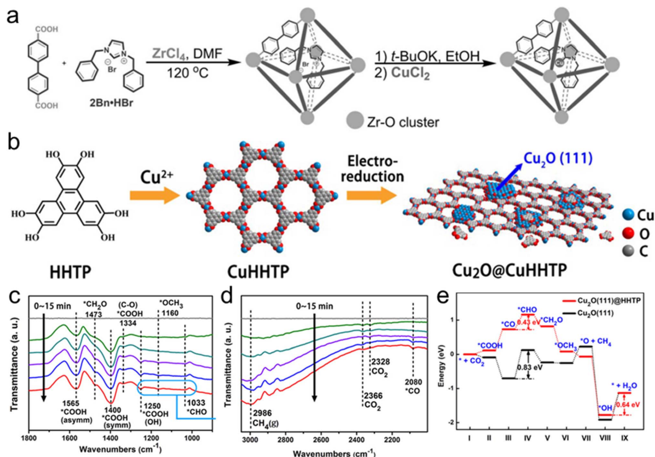
Fig. 15 (a) Synthetic scheme of 2Bn-Cu@UiO-67. Reproduced with permission. 188 Copyright 2021 Wiley. (b) Solvothermal synthesis of CuHHTP and preparation of \text{Cu}_2\text{O}@CuHHTP via electrochemical treatment of CuHHTP at -1.2 V for 30 min. (c and d) Operando ATR-FTIR spectra on \text{Cu}_2\text{O}@CuHHTP collected at -1.4 V vs. RHE in \text{CO}_2 saturated 0.1 M KCl/0.1 M \text{KHCO}_3 electrolyte. (e) Free-energy diagrams of the e\text{CO}_2\text{RR} to \text{CH}_4 for \text{Cu}_2\text{O}(111)@HHTP (red line) and the pristine \text{Cu}_2\text{O}(111) crystal plane (black line). Reproduced with permission. 190 Copyright 2020 Wiley.
