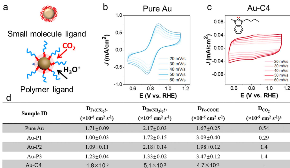
Fig. 2 (a) Schematic illustration of small molecule and polymer ligand modified metal nanocatalysts for \text{CO}_2 and proton transport. Cyclic voltammetry scans of (b) AuNPs and (c) Au-C4 measured with 5\text{ mM K}_3\text{Fe}(\text{CN})_6 at various scan rates. Reproduced with permission. 86 Copyright 2025 American Chemical Society. (d) Summary of the diffusion coefficient ( D ) using various probe molecules including \text{Fe}(\text{CN})_6^{3-} , \text{Ru}(\text{NH}_3)_6^{3+} , \text{Fc-COOH} , and \text{CO}_2 . P1–P3: N -heterocyclic carbene (NHC)-functionalized poly(ethylene oxide) (NHC-PEO- \text{HCO}_3^- , P1), NHC-PS- \text{HCO}_3^- (P2), and block copolymer NHC-PEO- b -PS- \text{HCO}_3^- (P3). Reproduced with permission. 111 Copyright 2023 The Royal Society of Chemistry.
