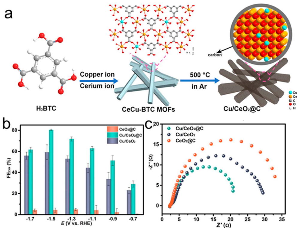
Fig. 16 (a) Schematic illustration for the synthesis of \text{Cu/CeO}_2@\text{C} . (b) Product FE of \text{Cu/CeO}_2@\text{C} at varied applied potentials. (b) The comparison of \text{CH}_4 selectivity. (c) Nyquist plots of \text{Cu/CeO}_2@\text{C} , \text{Cu/CeO}_2 and \text{CeO}_2@\text{C} . Reproduced with permission. 211 Copyright 2023 American Chemical Society.
