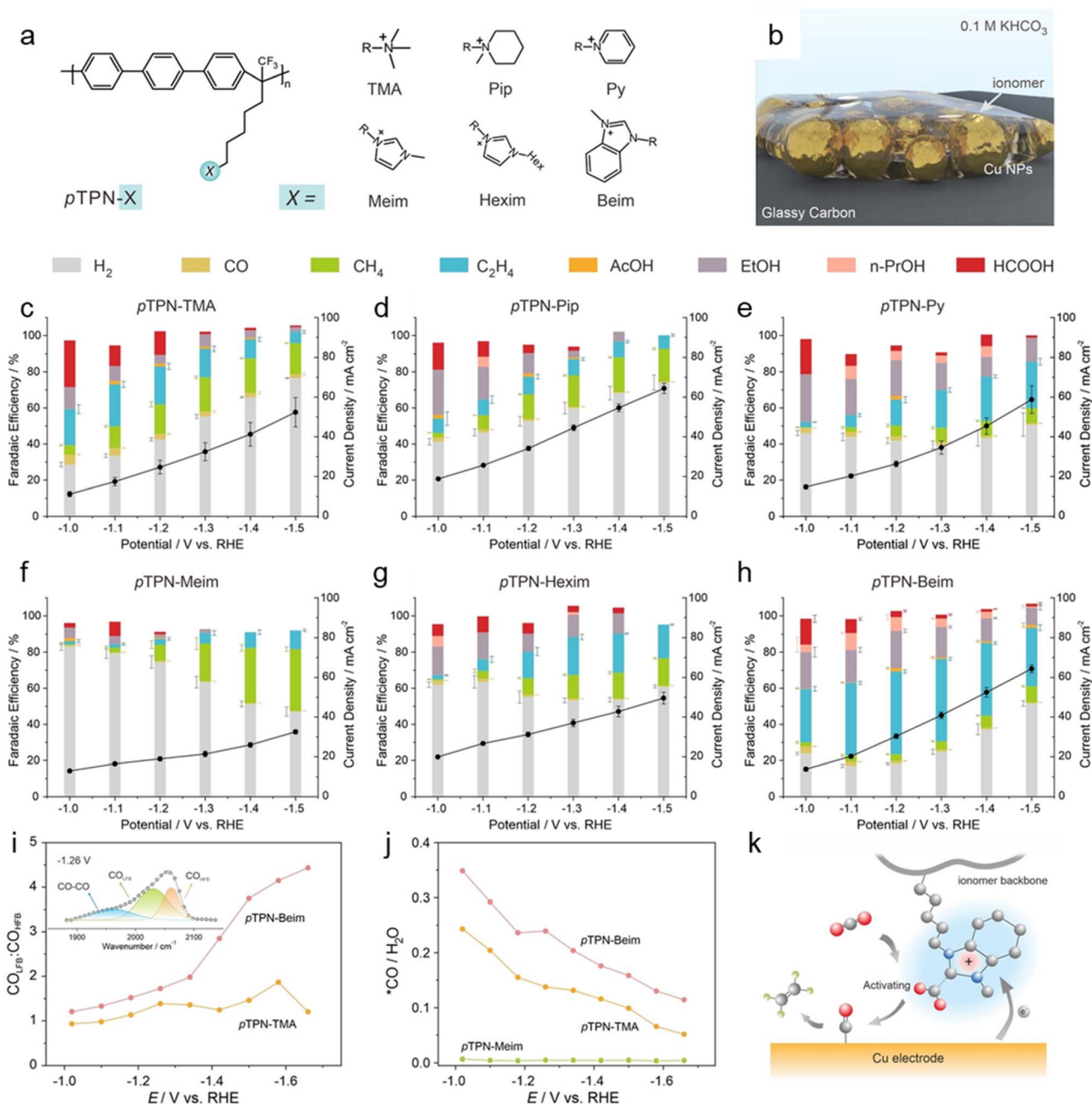
Fig. 11 (a) Structural illustration of p TPN-X ionomers. (b) Scheme of the p TPN-X-modified Cu electrode (Cu/ p TPN-X) for the \text{eCO}_2\text{RR} . (c)–(h) Product distribution and current densities over the Cu/ p TPN-X electrodes. (i) Ratios of \text{CO}_{\text{LFB}} to \text{CO}_{\text{HFB}} band intensity against the applied potentials. The inset shows typical peak decomposition of the ATR-SEIRAS acquired on Cu/ p TPN-Beim at -1.26 V. (j) Ratios of \nu(\text{CO}_\text{L}) to \nu(\text{H}_2\text{O}) band intensity against the applied potentials. (k) Schematic illustration of the \text{Beim}^+ cation-enhanced \text{CO}_2\text{RR} toward \text{C}_2\text{H}_4 production. Reproduced with permission. 154 Copyright 2023 Wiley.
