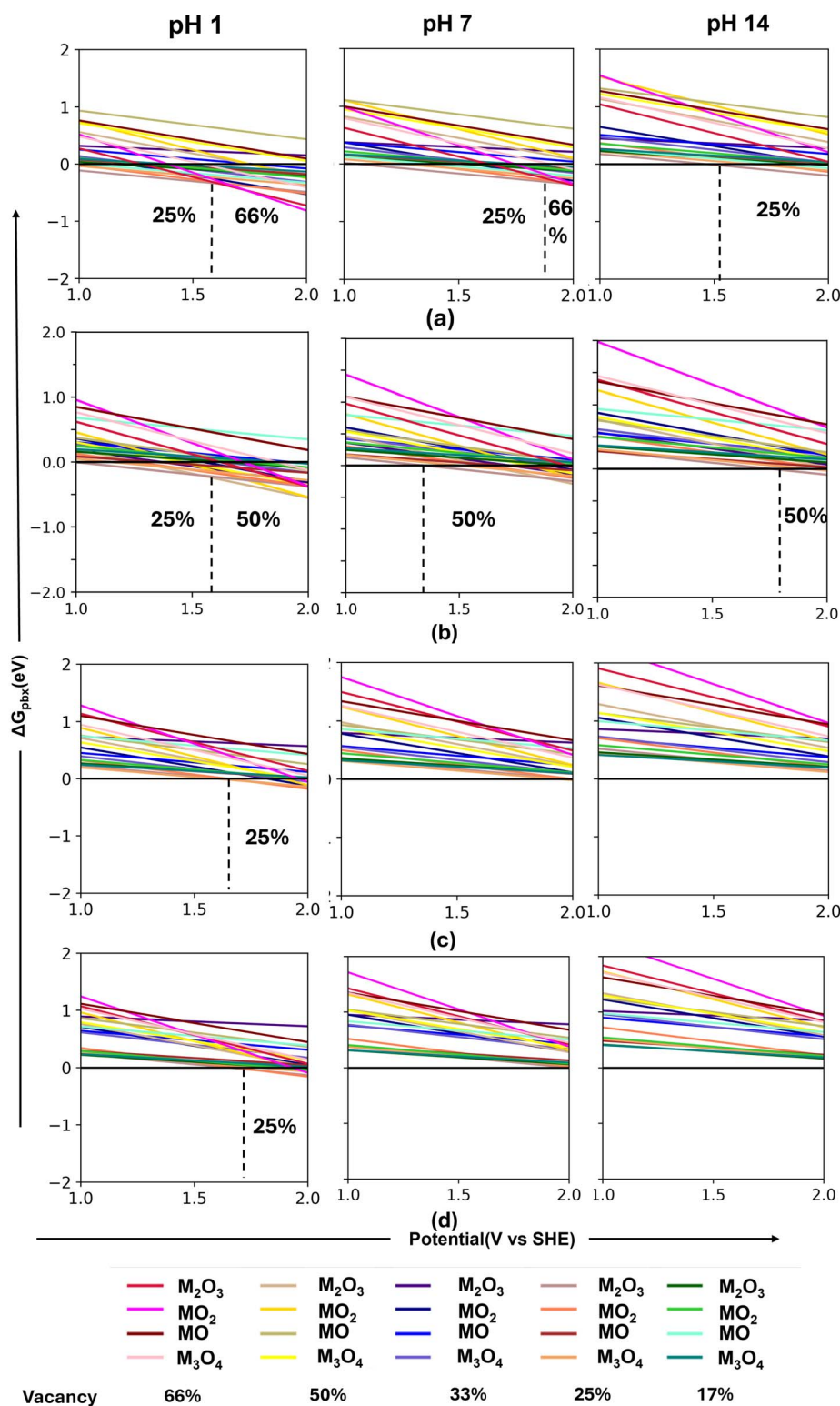
Fig. 2 (a)–(d) Illustrate the Pourbaix diagrams for \text{SrMnO}_3 , \text{SrFeO}_3 , \text{SrCoO}_3 , and \text{SrNiO}_3 , respectively, evaluated at pH 1, 7 and 14 under an applied potential range from 1.0 to 2.0 V. These diagrams include various corresponding metal oxides such as \text{MO} , \text{MO}_2 , \text{M}_2\text{O}_3 , and \text{M}_3\text{O}_4 , and consider different metal vacancy compositions of 17%, 25%, 33%, 50% and 66%. Across all compositions and materials, the Pourbaix plots consistently denote enhanced thermodynamic stability associated with a 66%, 25% metal-site vacancy for \text{SrMnO}_3 , 25% and 50% metal-site vacancy for \text{SrFeO}_3 , 25%, and pristine surfaces for \text{SrCoO}_3 and \text{SrNiO}_3 . The inset below shows the colour scheme considered to denote the different dissolution products.
