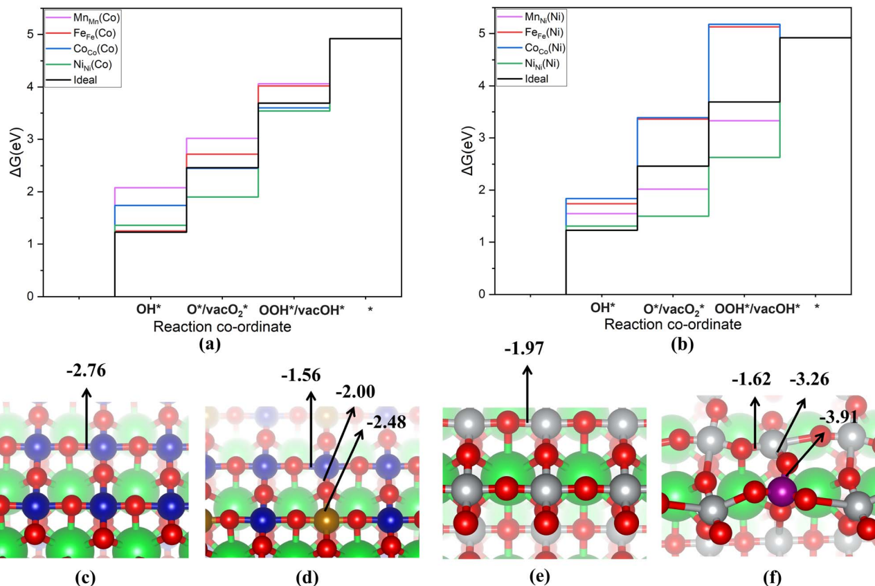
Fig. 6 (a) and (b) Free energy diagrams (FEDs) for the most favorable reaction pathways on various doped perovskite surfaces of \text{SrCoO}_3 and \text{SrNiO}_3 . The black lines represent an ideal catalyst surface, with each reaction step assigned an energy of 1.23 eV. The FEDs in purple, red, blue, and green correspond to Mn-, Fe-, Co-, and Ni-doped surfaces, respectively. (a) shows the FEDs for \text{SrCoO}_3 with different dopants, and (b) shows those for \text{SrNiO}_3 with different dopants. (c) and (d) The ICOHP values for undoped \text{SrCoO}_3 and Fe-doped \text{SrCoO}_3 , respectively. (e) and (f) Show the ICOHP values for undoped \text{SrNiO}_3 and Mn-doped \text{SrNiO}_3 .
