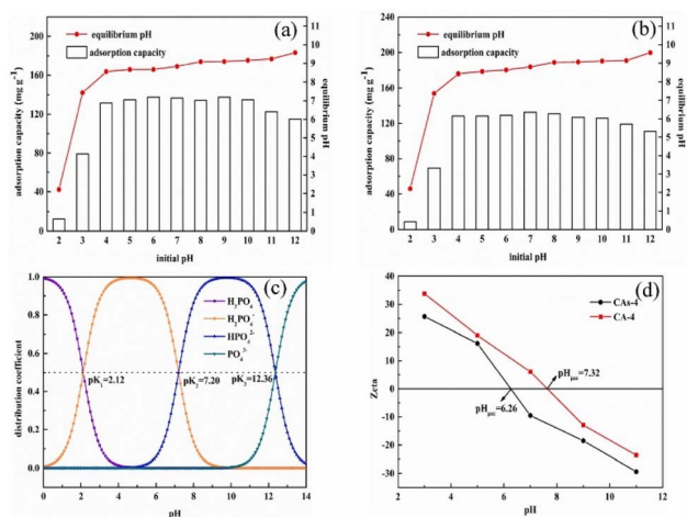
Fig. 4 (a) Effect of pH on CAs-4 adsorption of phosphate and final pH, (b) effect of pH on CA-4 adsorption of phosphate and final pH, (c) the phosphate speciation with varying pH value, (d) the zeta potential of CAs-4 and CA-4. Reprinted from ref. 53 with permission from Elsevier, Copyright 2022.
