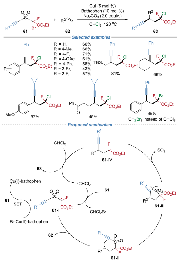
Scheme 22 Radical monofluoroalkylative alkylation of alkenes.
