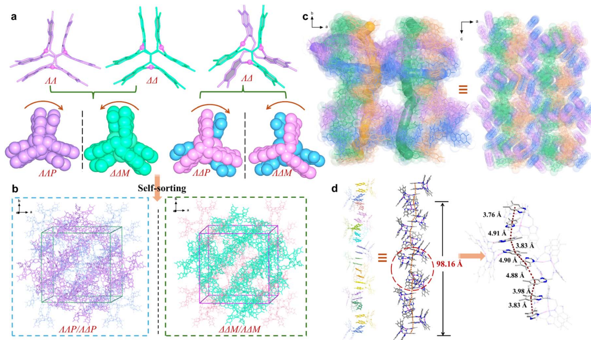
Fig. 2 Crystal structure of 3a . (a) \Delta\Delta P^- , \Delta\Delta M^- , \Delta\Delta P^- , and \Delta\Delta M^- -[Ag 3 L 3 ] 3+ in 3a-P or 3a-M . (b) Narcissistic self-sorting of [Ag 3 L 3 ] 3+ forming chiral structures of 3a-P and 3a-M . (c) One of the channels along the c axis constructed by quadruple helices in 3a-P . (d) One of the \pi -stacked helical columns with a pitch of \sim 98.16 Å.
