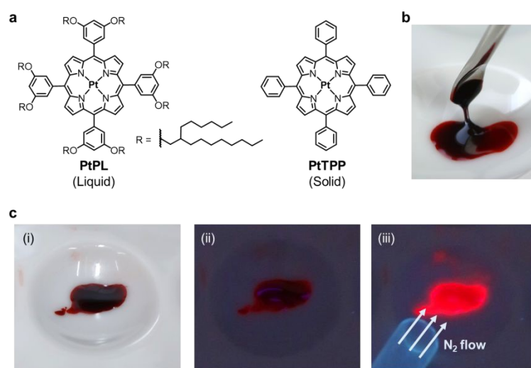
Figure 1. (a) Chemical structures of Pt(II) porphyrins; alkylated liquid ( PtPL ) and solid PtTPP used in this study. (b) Photograph of PtPL at 20 °C showing solvent-free liquid appearance. (c) Phosphorescent property of PtPL observed under daylight in air (i), under UV light in air (ii), and under UV light with N 2 flow (iii).
