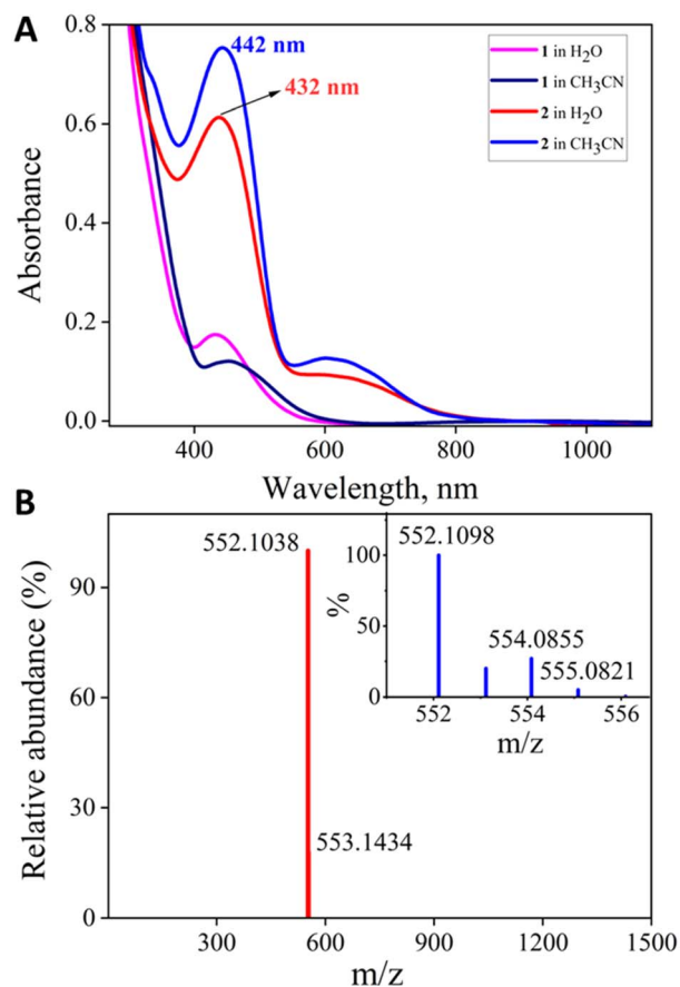
Fig. 2 (A) UV-vis spectra of 2 , both in 100% \text{CH}_3\text{CN} and water from 1 at RT. (B) Negative mode HRMS spectrum of 2 (0.05 mM) in water and mass spectrum of 2 in \text{H}_2\text{O}^{18} (inset).
