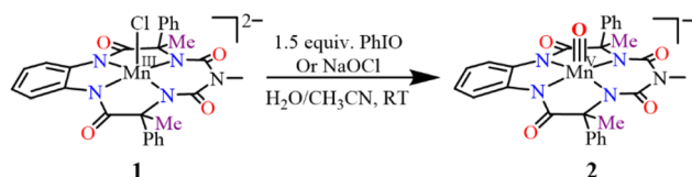
Scheme 1 Schematic diagram for the synthesis of complex (\text{Et}_4\text{N})[\text{Mn}^{\text{V}}(\text{O})(\text{Ph,Me-bTAML})] , 2 from 1 .
