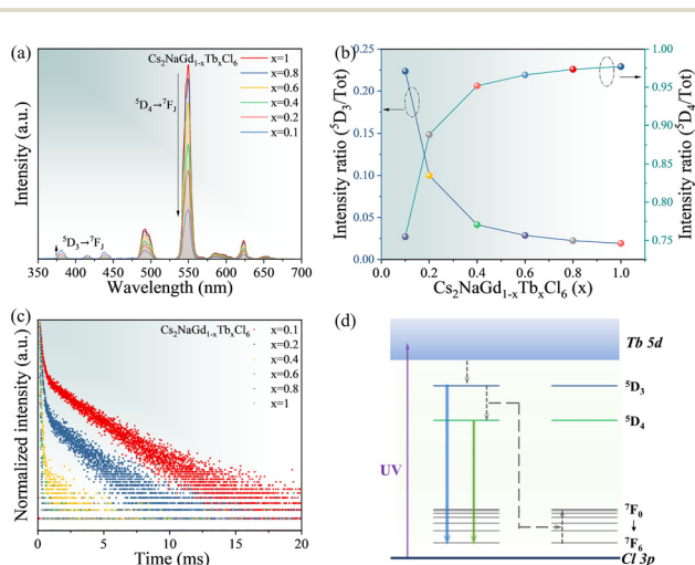
Fig. 2 (a) PL spectra of Cs_2NaGd_{1-x}Tb_xCl_6 under an excitation wavelength of 275 nm. (b) The emission ratio from ^5D_3 and ^5D_4 levels over total emission. (c) Photoluminescence decay curves for the ^5D_3 level (437 nm). (d) Energy-level diagram for Tb^{3+} ions in Cs_2NaGd_{1-x}Tb_xCl_6 showing a possible route of luminescence quenching and cross-relaxation.
