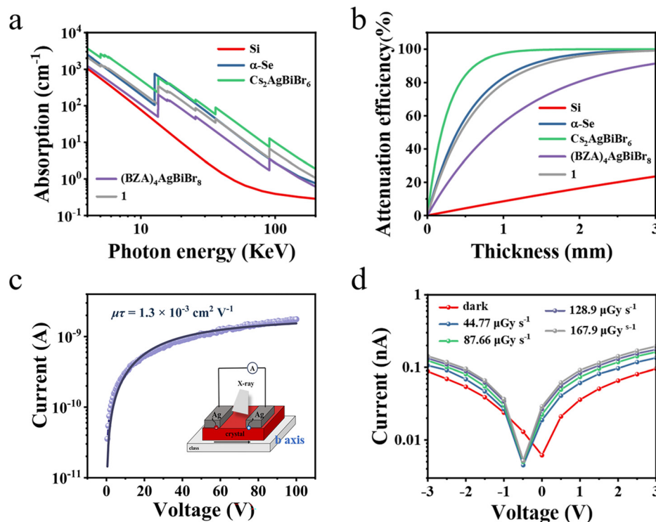
Fig. 2 (a) X-ray absorption spectra and (b) corresponding attenuation efficiencies of Si, \alpha -Se, \text{Cs}_2\text{AgBiBr}_6 , (\text{BZA})_4\text{AgBiBr}_8 , and 1 . (c) Bias-dependent X-ray conductivity of the 1 SC device. (d) I – V curves of the 1 device along the b -axis in the dark and under X-ray irradiation.
