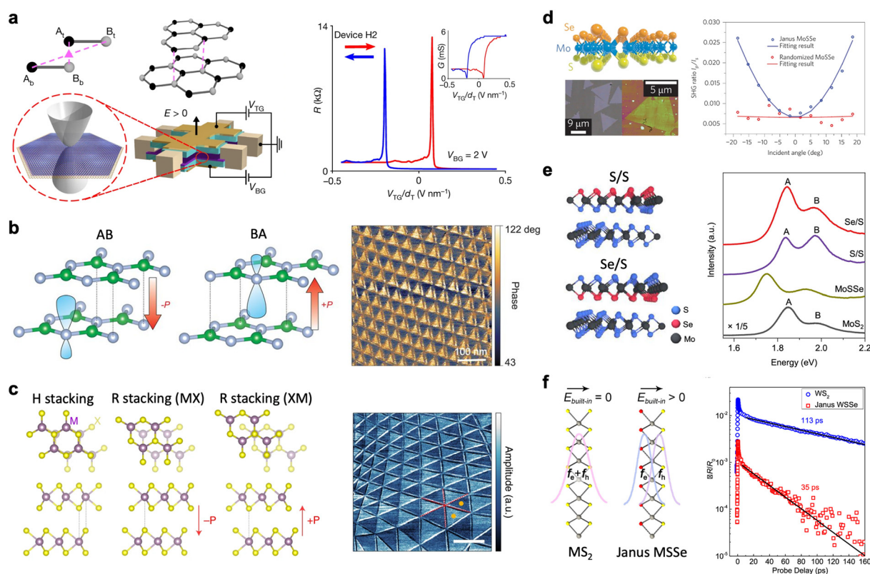
Fig. 3 (a) (Left) Schematic of atomic structure of Bernal-stacked bilayer graphene and device structures with top and bottom gates. (Right) Gated-tuned resistance of the hysteretic devices; reproduced from ref. 38 with permission from Springer Nature, copyright 2020. (b) (Left) Schematic of different atomic arrangement for AB- and BA-stacked hBN homobilayer with induced ferroelectricity. (Right) Vertical PFM phase image of twist bilayer hBN; reproduced from ref. 40 with permission from Science, copyright 2021. (c) (Left) Atomic structure of H-stacked, R-stacked (MX and XM) bilayer TMD. (Right) Amplitude image of vertical PFM on MoSe 2 ; reproduced from ref. 44 with permission from Springer Nature, copyright 2022. (d) (Left) Atomic structure, optical microscopy, and atomic force microscopy images of Janus MoSSe. (Right) SHG intensity as a function of incident angle; reproduced from ref. 51 with permission from Springer Nature, copyright 2017. (e) (Left) Atomic structure of heterobilayers with S/S and Se/S interface. (Right) PL spectra of MoS 2 monolayer, MoSSe monolayer, and twisted heterobilayers with S/S and Se/S interface; reproduced from ref. 52 with permission from American Chemical Society, copyright 2021. (f) (Left) Side view of MS 2 and Janus MSSe. (Right) Pump-probe differential reflectance signal versus the probe photon energy for Janus WS 2 and WSSe; reproduced from ref. 53 with permission from American Chemical Society, copyright 2021.
