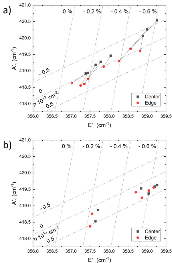
Fig. 3 A comparison of E' and A_1^g Raman positions at the center and the edge of the WS 2 flakes. (a) WS 2 grown on reconstructed sapphire and (b) WS 2 grown on standard sapphire. Connecting lines between data point in (a) indicate data from the same crystal. The horizontal dotted lines with a slope of 0.55 indicate constant doping level and vertical dotted lines with a slope of 6.16 indicate constant strain. The point with neutral doping and strain is \omega(E') = 356.7 \text{ cm}^{-1} and \omega(A_1^g) = 418.5 \text{ cm}^{-1} . The slopes and the neutrality point are based on previous work by Lee et al. 36
