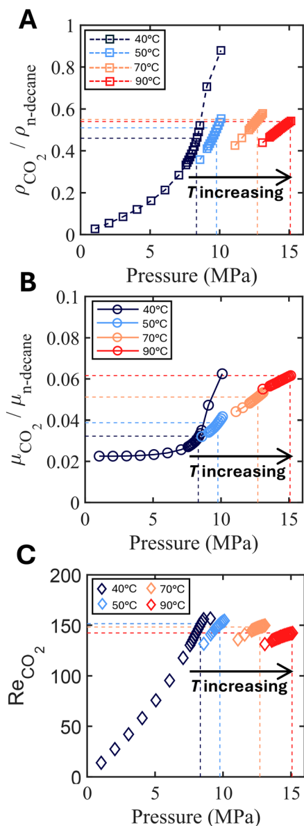
Fig. 12 Variation of dimensionless parameters at different temperatures and pressures. (A) The density ratio \rho_{\text{CO}_2} / \rho_{n\text{-decane}} , (B) the viscosity ratio \mu_{\text{CO}_2} / \mu_{n\text{-decane}} , and (C) the Reynolds number of \text{CO}_2 .
