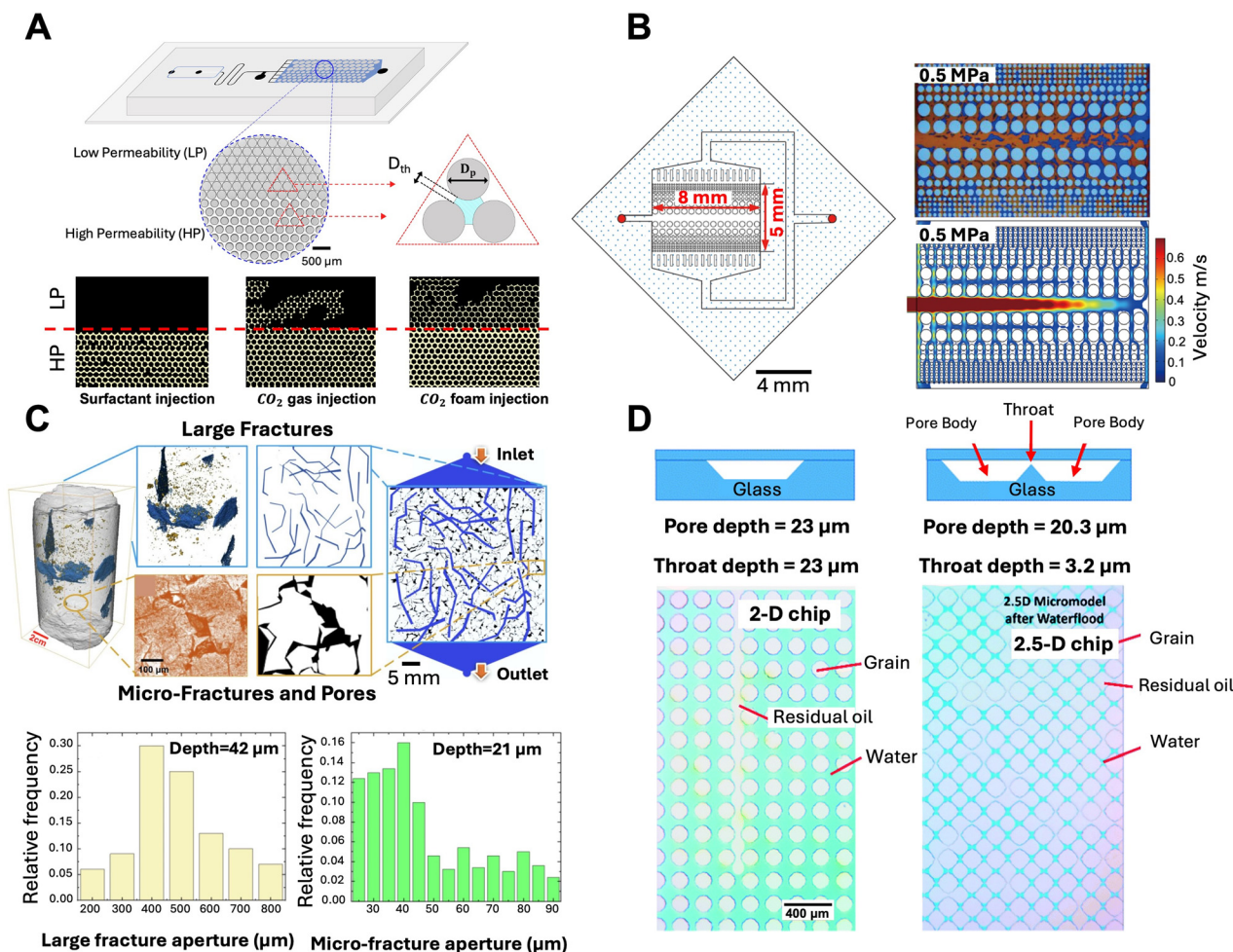
Fig. 5 Heterogeneous microfluidic pore networks. (A) Fluid displacement in a dual-permeability PDMS chip with circular pillars (210 \mu m , 250 \mu m ) and throats (60 \mu m , 21 \mu m ); depth 100 \mu m . Oil and pillars are black, displacing fluids yellow (adapted with permission from Moradpour and Tsai. 121 Copyright © 2025 Royal Society of Chemistry). (B) Fracturing fluid propagation in a multi-permeability chip simulating fracture-matrix zones. Pillars: 200, 100, 50 \mu m ; throats: 125, 80, 70 \mu m ; central fracture: 500 \mu m ; depth 30 \mu m . Right: Guar gum fluid (blue), oil (brown), and velocity map at \Delta P = 0.5 MPa (adapted with permission from Da et al. 122 Copyright © 2022 KeAi Elsevier). (C) Oil displacement by CO_2 in a fractured micromodel replicated from carbonate rock micro-CT. Glass chip patterned and etched to include large and micro fractures; mean depths 42 \mu m and 21 \mu m (adapted with permission from Lv et al. 123 Copyright © 2022 Elsevier). (D) Oil displacement by water in 2D and 2.5D hydrophilic micromodels. N -Octane (gray) displaced by dyed water (blue); capillary snap-off observed only in 2.5D chip (adapted with permission from Xu et al. 124 Copyright © 2017 Royal Society of Chemistry).
