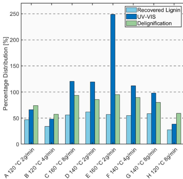
Fig. 5 Comparison of lignin extraction obtained from different processing conditions including: lignin recovery from the purification process (recovered lignin), lignin yield from calibrated UV-Vis and lignin yield calculated based on the lignin content in the extraction residue (delignification).
