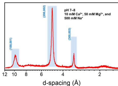
Fig. 5 The formation of todorokite in the presence of multiple cations. Although the concentrations of Mg^{2+} and Ca^{2+} are much lower than that of Na^+ in the seawater mimicked solution, the XRD result shows the formation of todorokite, suggesting the feasibility of the reaction in environmental systems.
