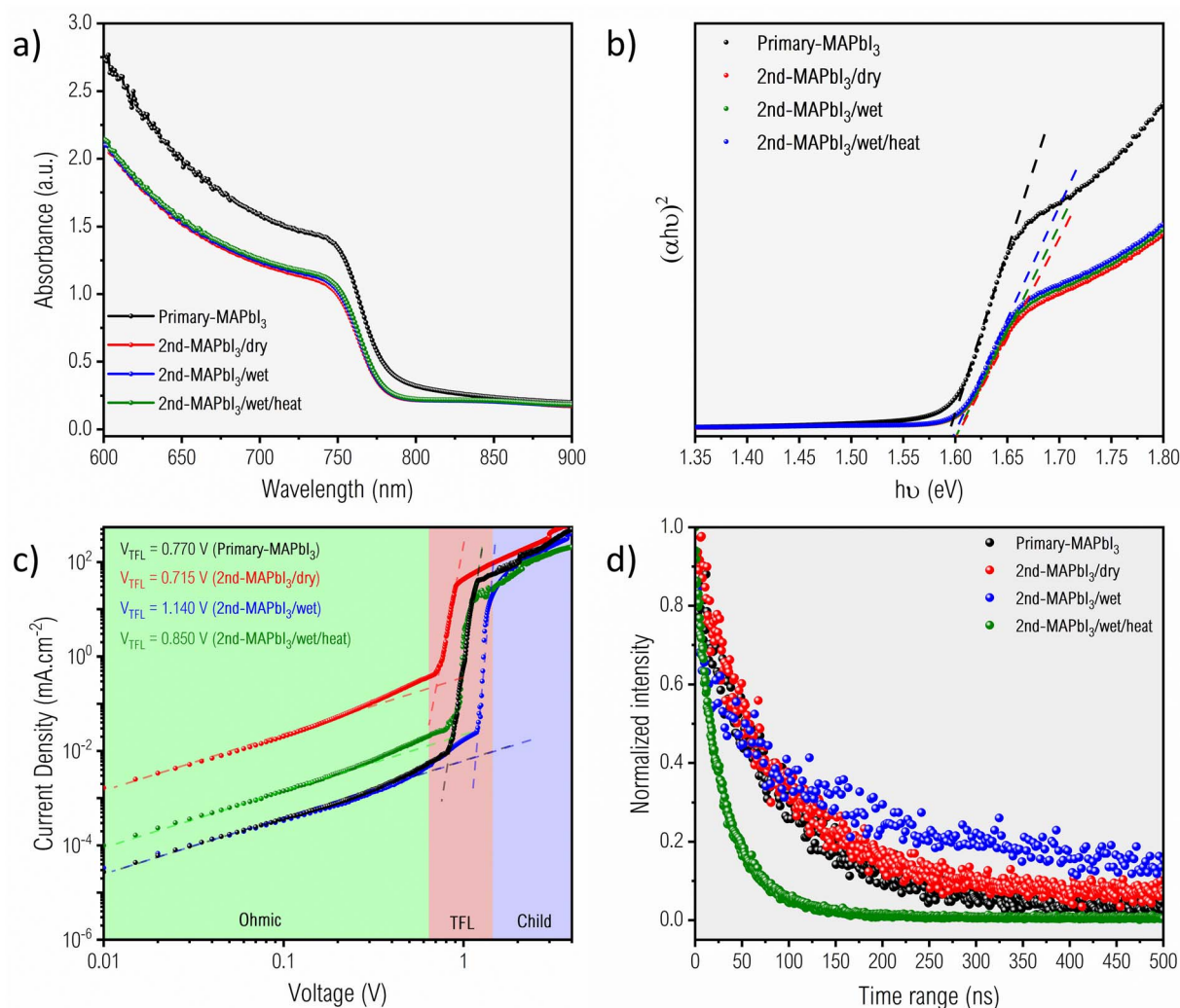
Fig. 8 (a) UV-vis absorption spectra, (b) Tauc-plot, (c) the SCLC curves and (d) the TRPL spectra of the glass/Al 2 O 3 /PVSK film of Primary-MAPbI 3 , 2nd-MAPbI 3 /dry, 2nd-MAPbI 3 /wet and 2nd-MAPbI 3 /wet/heat films.
