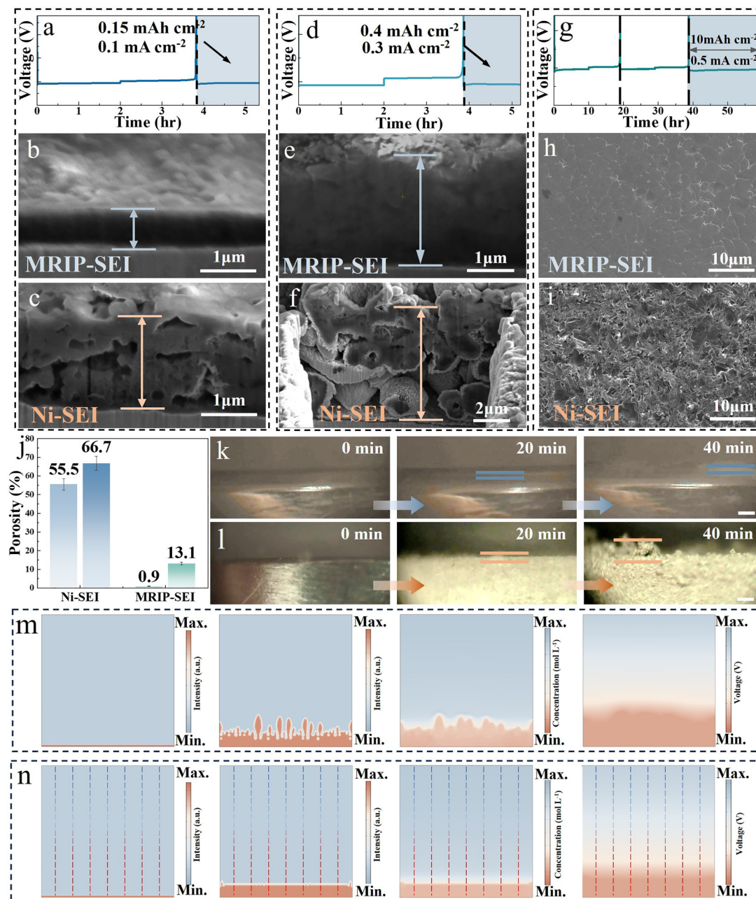
Fig. 5 Deposition behaviors on various current collectors. (a) Charge/discharge profiles and corresponding FIB-SEM images with (b) the MRIP-SEI and (c) the Ni-SEI at 0.1 \text{ mA cm}^{-2} . (d) Charge/discharge profiles and corresponding FIB-SEM images with (e) the MRIP-SEI and (f) the Ni-SEI at 0.3 \text{ mA cm}^{-2} . (g) Charge/discharge profiles and corresponding SEM images with (h) the MRIP-SEI and (i) the Ni-SEI at 0.5 \text{ mA cm}^{-2} . (j) Comparison of porosity of lithium deposition layers induced by different current collectors. Morphological evolution of electrodeposited Li characterized by real-time optical microscopy with (k) the MRIP-SEI and (l) the Ni-SEI. Phase field simulation results of lithium deposition induced by (m) heterogeneous nucleation (Ni-SEI) and (n) uniform nucleation (MRIP-SEI).
