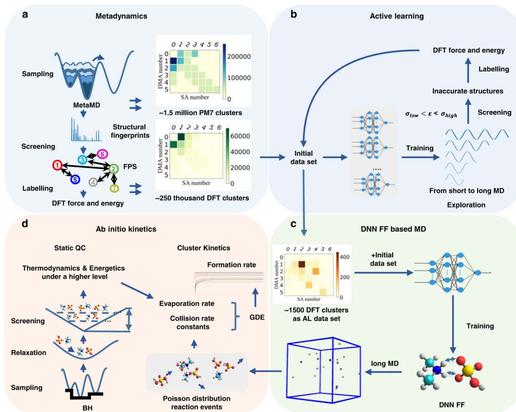
Fig. 11 A general workflow towards fully ab initio simulation of atmospheric aerosol nucleation. It includes the steps to prepare the data set for training a deep neural network-based force field (DNN-FF), to apply DNN-FF by molecular dynamics (MD), to derive collision rate coefficients from MD, and to couple collision rate coefficients with cluster dynamics model for studying atmospheric aerosol nucleation. (a and b) Shows the metadynamics and active learning techniques used to prepare a data set for the deep neural network, respectively. (c) DNN-FF-driven MD. (d) Cluster dynamics simulation based on MD-derived collision rate coefficients and static quantum chemistry (QC) calculation-derived evaporation rates. Adapted from Jiang et al. , 2022. 21 Adapted from ref. 21 with permission from the Springer Nature, copyright 2022. Permission conveyed through Copyright Clearance Center.
