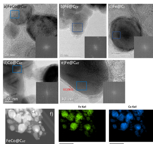
Fig. 2 Selected TEM images of (a) FeCo@C HT , (b) Fe@C CP , (c) Fe@C I , (d) Co@C HT , and (e) Fe@C HT magnetic nanoparticles. HAADF-STEM images of (f) FeCo@C HT and EDS mapping of Fe (green) and Co (blue) in FeCo@C HT .
