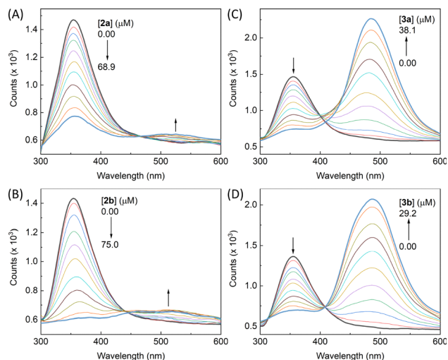
Fig. 12 Fluorescence spectra tracking the titration of bovine serum albumin (10 μM) with (A) 2a , (B) 2b , (C) 3a , and (D) 3b in 0.1 M phosphate buffer (pH 7.4). Excitation wavelength ( \lambda_{\text{ex}} ): 277 nm. Arrows denote spectral changes with increasing fluorophore concentration.
