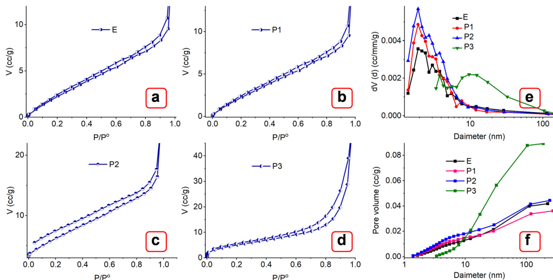
Fig. 3 N_2 adsorption curves of MOFs (a) E, (b) P1, (c) P2, (d) P3. BJH pore volume plots of MOFs (e) and (f).
