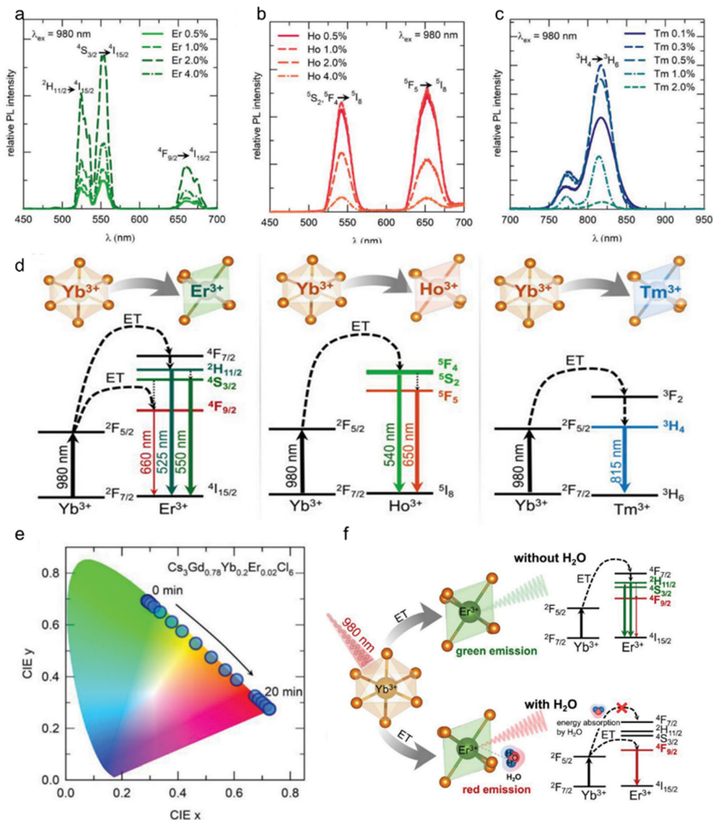
Fig. 7 (a) Different Er 3+ dopant concentrations in Cs 3 Gd 1-x-y Yb x Er y Cl 6 PCs under 980 nm laser excitation; (b) different Ho 3+ dopant concentrations in Cs 3 Gd (1-x-y) Yb x Ho y Cl 6 PCs upon 980 nm laser excitation; (c) different Tm 3+ dopant concentrations in Cs 3 Gd (1-x-y) Yb x Tm y Cl 6 PCs upon 980 nm laser excitation. (d) Mechanism of energy transfer from Yb 3+ to Er 3+ , Ho 3+ , and Tm 3+ ions for UCL. (e) CIE coordinates of UCL from Er 3+ , Ho 3+ , and Tm 3+ . (f) The UCL mechanism of Cs 3 GdCl 6 :Yb 3+ , Er 3+ PCs in the presence and absence of water molecules. Reproduced with permission from ref. 55. Copyright 2023, Wiley.
