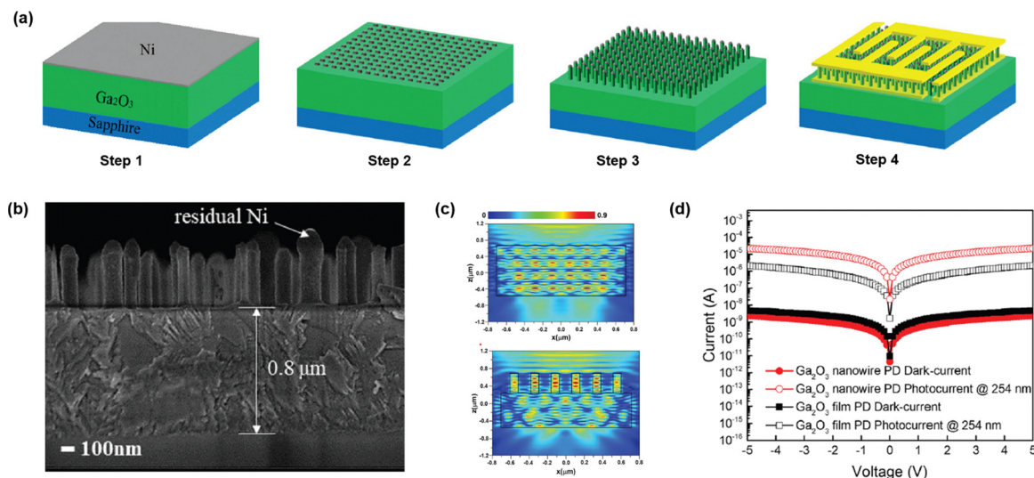
Fig. 16 (a) Schematic of the fabrication process steps of \beta - \text{Ga}_2\text{O}_3 NW PD. (b) FESEM image of the \beta - \text{Ga}_2\text{O}_3 NW array. Comparison of (c) light field intensity of NW and flat surface \beta - \text{Ga}_2\text{O}_3 . (d) I - V characteristics of PD with and without a NW array. Reproduced with permission. 123 Copyright 2020, De Gruyter.
