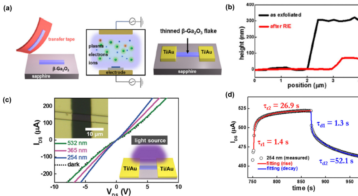
Fig. 17 (a) Schematic of the fabrication process steps of \beta - \text{Ga}_2\text{O}_3 micro-flakes PD. (b) AFM image showing thinning of the flakes. (c) I - V characteristics and (d) transient response of PD. Reproduced with permission. 45 Copyright 2017, AIP Publishing.
