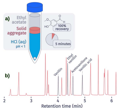
Fig. 2 Development of a lignin quantification method. (a) Illustration of the spontaneous formation of a solid aggregate at the phase-boundary during extraction, which allowed for a fast, yet quantitative extraction. (b) Eighteen plausible monomeric lignin products were separated in 6 minutes. The analytes of interest in this study are highlighted, demonstrating a sufficiently high resolution to avoid peak interference even at higher concentrations. Remaining details are found in Table S12.
