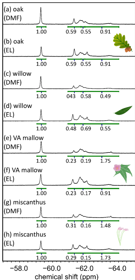
Fig. 4 Stacked plot of 1D low-field 19 F NMR spectra of derivatized pyrolysis oil produced from oak (a) in DMF and (b) in EL, produced from willow (c) in DMF and (d) in EL, produced from Virginia mallow (e) in DMF and (f) in EL, and produced from miscanthus (g) in DMF and (h) in EL. All samples contain the internal standard, 3-(trifluoromethoxy) benzoic acid.
