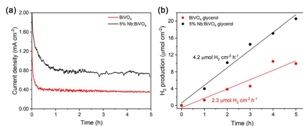
Fig. 8 (a) Chronoamperometry graphs of BiVO 4 and 5% Nb : BiVO 4 in crude glycerol 10% v/v in K 2 SO 4 0.1 M under 1.0 V vs. RHE and 100 mW cm -2 AM 1.5 G illumination. (b) H 2 evolution from an average of 3 chronoamperometry experiments for BiVO 4 and 5% Nb : BiVO 4 photoanodes.
