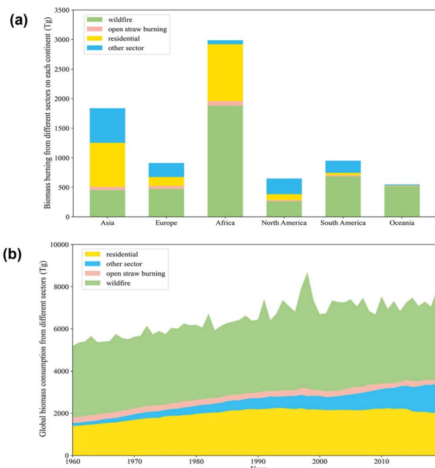
Fig. 6 (a) Continent-wise statistics of the extent of biomass destroyed by burning (in 2019), (b) global trend of total biomass burnt annually over the decades, reproduced from ref. 111 with permission from Elsevier, copyright 2024.
