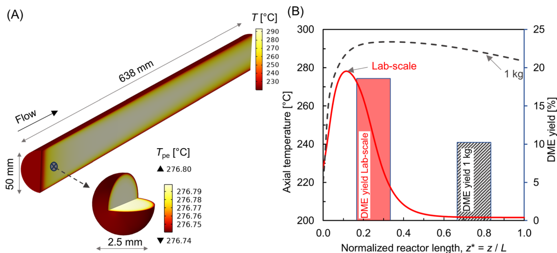
Fig. 15 (A) 3-D visualization of temperature distribution in 1 kg (0.86 kg CZA and 0.14 kg \text{Al}_2\text{O}_3 ) reactor; (B) comparison of centerline temperature profile (line plot, left y-axis) and DME yield (histogram, right y-axis) between lab-scale ( 3.57 \times 10^{-3}\text{ kg} ) and 1 kg reactor. The process conditions are: T_{in} = 220\text{ }^{\circ}\text{C} , \text{WHSV} \sim 1.1\text{ h}^{-1} , T_{in} - T_w = 20\text{ }^{\circ}\text{C} , p = 10\text{ bar} .
