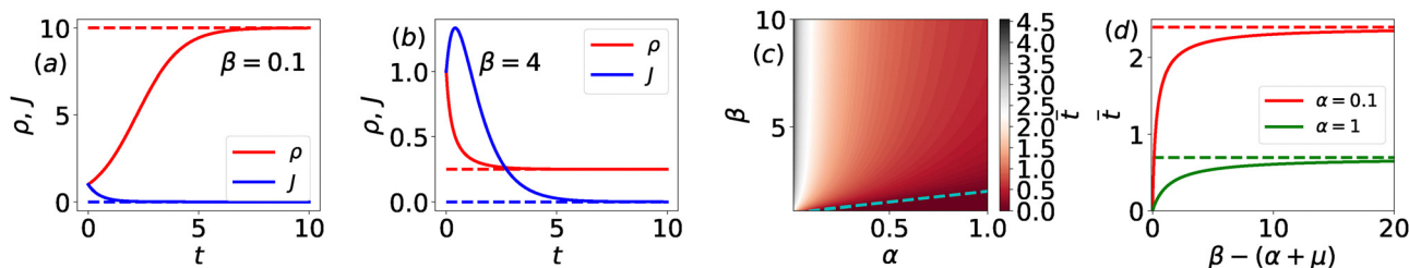
Fig. 3 Mean-field approximation. (a) Time evolution of density \rho and current J for \beta = 0.1 ( \alpha = \mu = \nu = 1 ). The dashed lines indicate the stationary values. (b) The current J develops a peak at \bar{t} for increasing values of \beta (here \beta = 4 and \alpha = \mu = \nu = 1 ). (c) Contour plot \bar{t}(\alpha, \beta) . Below the dashed line \bar{t} = 0 . (d) \bar{t} as a function of \beta for \alpha = 0.1, 1 (see legend). The dashed lines indicate the asymptotic values \beta \rightarrow \infty .
