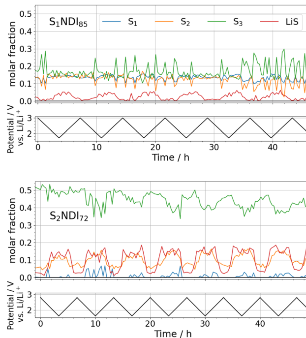
Fig. 6 Evolution of molar fractions of different sulfur strand lengths and of the signal of lithium sulfur bonds ( \text{LiS} ) over several CV cycles, determined by a linear combination analysis of operando NEXAFS spectra of \text{Li-S}_1\text{NDI}_{85} and \text{Li-S}_2\text{NDI}_{72} half-cells. S_1 , S_2 and S_3 species are represented by DPS, DPDS and DMTS basis spectra and correspond to molar fractions of sulfur in mono-, di- and trisulfide strands, respectively. The \text{LiS} coefficient is proportional, but not equal to the molar fraction of lithium sulfur bonds.
