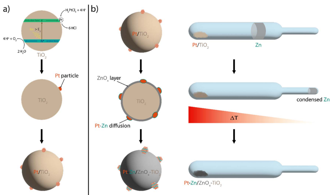
Fig. 1 Reaction scheme for the loading of TiO 2 nano powder (P25) with Pt co-catalyst particles via in situ photoreduction (a) and the consequent vapour–solid process (b) for the formation of intermetallic Pt–Zn co-catalysts.
