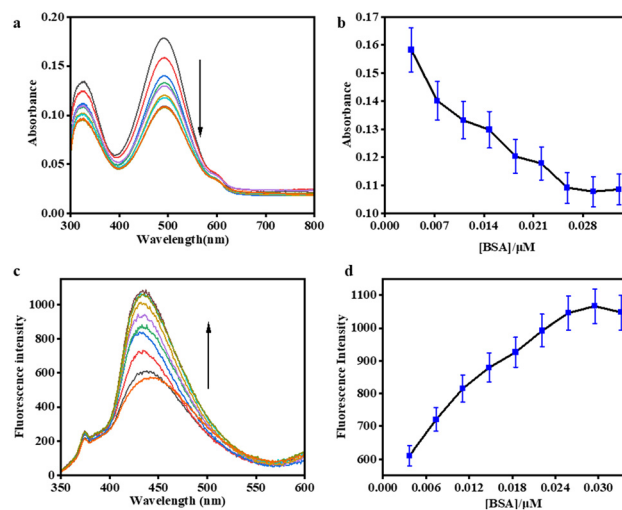
Fig. 8 (a) and (c) UV-vis and fluorescence of DSM ( c = 2.0 \times 10^{-5} M) upon titration with BSA ( c = 7.4 \mu M) in Tris-HCl buffer at pH 7.2 respectively. (b) and (d) Changes in concentration vs. intensity in UV-vis ( \lambda_{em} = 490 nm) and fluorescence spectra ( \lambda_{em} = 425 nm) respectively.
