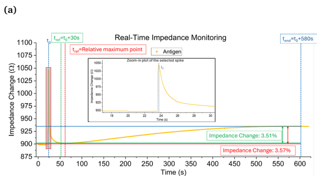
Fig. 3 An example of the data analysis methods using 1000 \text{ng mL}^{-1} SARS-CoV-2 spike protein samples. (a) Comparison of real-time impedance monitoring after pipetting 1 \times PBS, antibodies, and antigens. (b) Comparison of two analysis methods.
