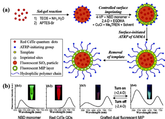
Fig. 31 (a) Fluorescence “turn-on” optosensing of herbicide in pure milk using a ratiometric fluorescent microsphere. (b) Fluorescent spectra and fluorescence colors of the polymerizable NBD monomer (in CH 3 CN, b1) and red CdTe QDs (in H 2 O, b2) as well as those of the grafted dual fluorescent 2,4-D-MIP (b3) and its mixture with 2,4-D (b4) in pure bovine milk. Reprinted with permission from ref. 261. Copyright 2020 Elsevier.
