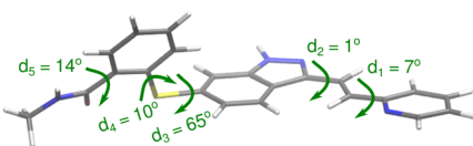
Fig. 3 The (a) form XLI molecular conformation is more folded than (b) the more typical form XXV one, leading to considerable deviations from planarity in dihedral angles d_4 and d_5 in particular.
