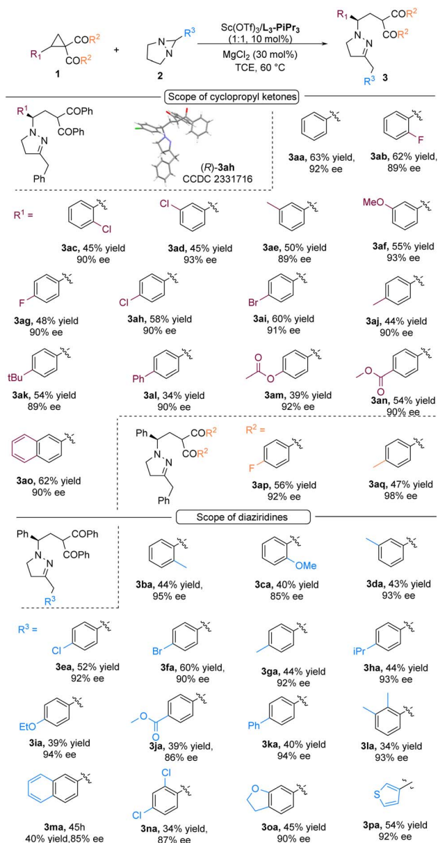
Scheme 3 Substrate scope. Unless otherwise noted, all reactions were performed with 1 (0.22 mmol), 2 (0.1 mmol), \text{Sc(OTf)}_3/\text{L}_3\text{-PiPr}_3 (1 : 1, 10 mol%), and \text{MgCl}_2 (30 mol%) in 1,1,2,2-tetrachloroethane (1.0 mL) at 60 °C for a defined amount of time. Isolated yields of the products were given. The ee values were determined by chiral UPCC analysis.
