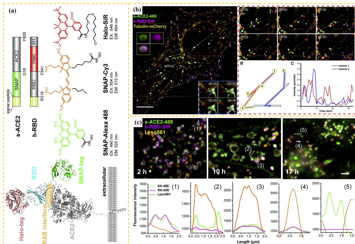
Fig. 49 (a) Schematic diagram of the design of RAB fusion protein, s-ACE2 and h-RBD constructs, and chemical structure of the Halo/SNAP probe. (b) SIM imaging of compound s-ACE2-488/h-RBD-SiR tracking the movement and maturation of vesicles in HeLa cells. (c) SIM imaging of the degradation process of compounds s-ACE2 and h-RBD in HeLa cells. Reprinted with permission from Elsevier, copyright 2023, as cited in ref. 122.
