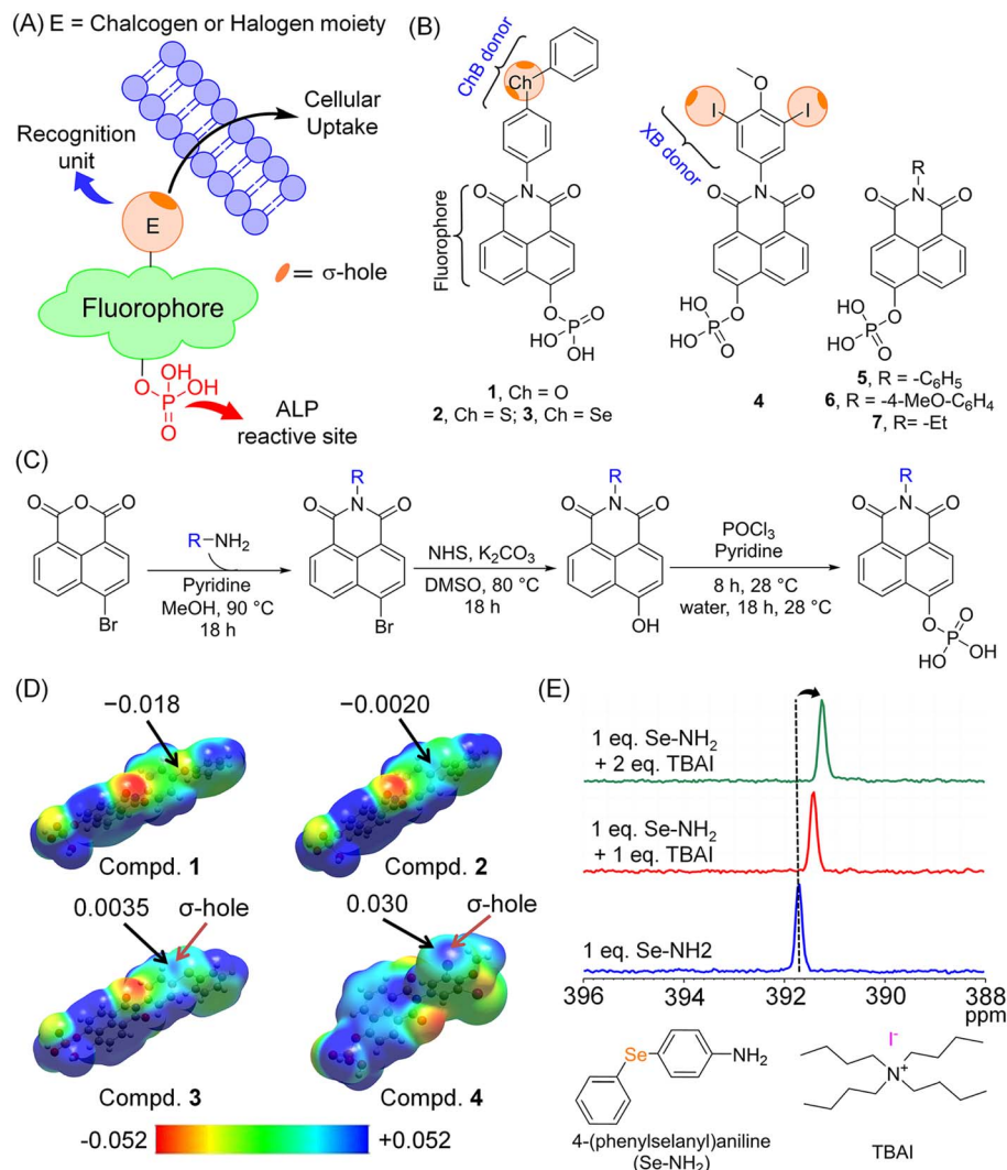
Fig. 1 (A) Design of ratiometric fluorescent compounds for monitoring ALP activity by attaching a phosphate group to a naphthalimide core along with a recognition moiety containing a σ-hole. (B) Structures of compounds 1–7 used in this study, featuring chalcogen and halogen atom substitutions. (C) General synthetic scheme for compounds 1–7 starting from 4-bromo-1,8-naphthalimide anhydride. (D) Electrostatic potential (ESP) diagrams for compounds 1–4, showing computed electrostatic potential maxima ( V_{S,max} ) at the σ-hole of chalcogen and halogen atoms (in a.u., iso value: 0.001 a.u.). (E) ^{77}\text{Se} NMR of 4-(phenylselenanyl)-aniline in the presence of different concentrations of tetrabutylammonium iodide in DMSO- d_6 .
