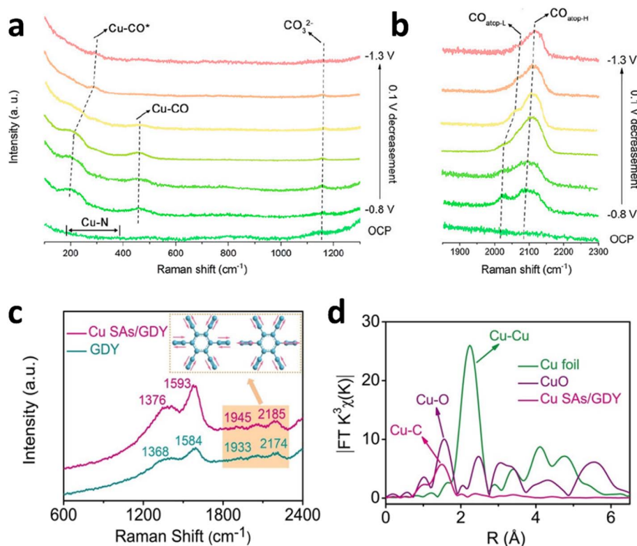
Fig. 8 In situ electrochemical SERS measurements for (a) low energy region and (b) high energy region for TWN-Cu 13.35 -600-SACs during the eCO 2 RR. (a) and (b) are reproduced from ref. 129 with permission from American Chemical Society, copyright 2023. (c) Raman spectra of pure GDY and Cu SAs/GDY. (d) FT EXAFS spectra of Cu SAs/GDY and Cu foil. (c) and (d) are reproduced from ref. 131 with permission from Wiley, copyright 2022.
