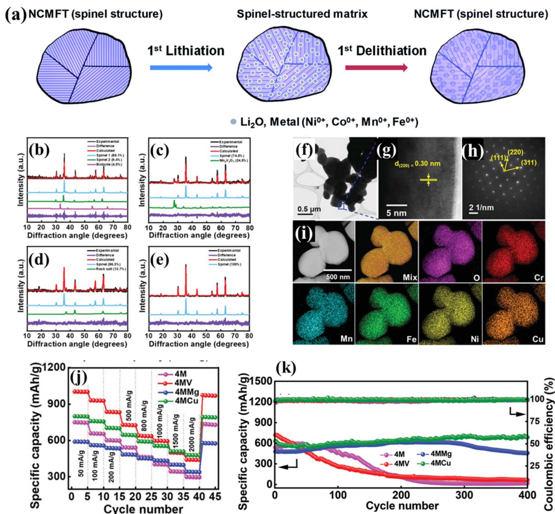
Fig. 10 HESs for LIBs. (a) Charge storage mechanism during initial lithiation and delithiation processes. 109 XRD patterns of (b) (\text{CrNiMnFe})_2\text{O}_4 (4M), (c) (\text{CrNiMnFeV})_3\text{O}_4 (4MV), (d) (\text{CrNiMnFeMg})_3\text{O}_4 (4MMg), and (e) (\text{CrNiMnFeCu})_3\text{O}_4 (4MCu); (f) TEM image, (g) high-resolution lattice image, (h) SAED pattern, and (i) HAADF image and EDS mapping of 4MCu; (j) comparative rate capability of various electrodes, and (k) cycling stability of various electrodes at 500 \text{ mA g}^{-1} for 400 cycles. Reproduced with permission. 108 Copyright 2022, John Wiley and Sons.
