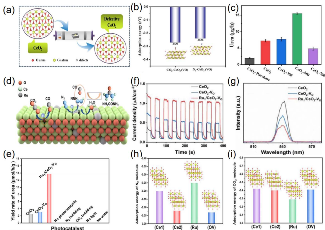
Fig. 13 (a) Schematic diagram of oxygen vacancy generation. (b) Adsorption energy of \text{N}_2 and \text{CO}_2 on \text{CeO}_2 with oxygen vacancy. (c) The urea formation rates of \text{CeO}_2 -purchase (commercial), \text{CeO}_2 , \text{CeO}_2 -300, \text{CeO}_2 -500 and \text{CeO}_2 -700 with all optical spectrum as light source. Reproduced with permission from ref. 63. Copyright 2023, Wiley-VCH. (d) Mechanism of the photocatalytic urea synthesis based on synergistic effects of the \text{Ru}_1/\text{CeO}_2 -VO. (e) The prepared materials and urea production efficiency under different conditions. (f) Photocurrent responses of \text{CeO}_2 , \text{CeO}_2 -VO, and \text{Ru}_1/\text{CeO}_2 -VO. (g) PL spectra of \text{CeO}_2 , \text{CeO}_2 -VO, and \text{Ru}_1/\text{CeO}_2 -VO. (h) \text{N}_2 adsorption energy of different sites. (i) \text{CO}_2 adsorption energy of different sites. Reproduced with permission from ref. 64. Copyright 2025, Wiley-VCH.
