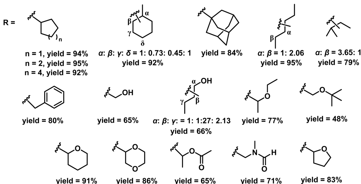
Scheme 98 Photocatalytic C–H alkylation of pyrimidines using \text{CHCl}_3 and 4CzIPN under blue LED light.
