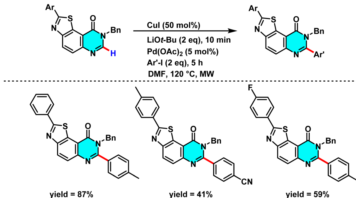
Scheme 12 \text{Pd}(\text{OAc})_2 -catalyzed activation of C(2)-H bonds in pyrimidine-containing structures.
