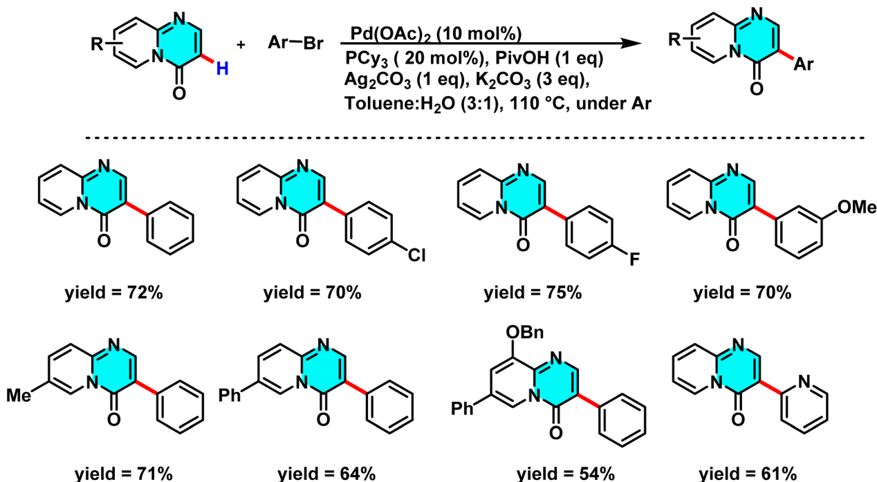
Scheme 7 Pd(II)-catalyzed synthesis of 3-aryl-pyrido[1,2- a ]pyrimidin-4-ones in the presence of Ag(I) as a co-catalyst.
