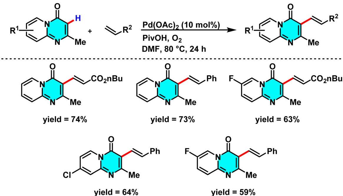
Scheme 3 Selective C(3)–H alkenylation of 2-methyl-4H-pyrido[1,2-a]pyrimidin-4-ones.
