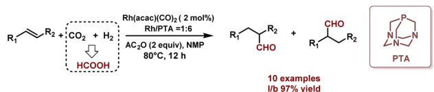
Fig. 14 Rh-PTA-catalyzed hydroformylation of olefins with CO 2 /H 2 .
