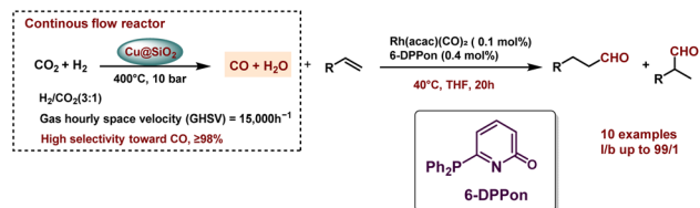
Fig. 13 Selective copper-catalyzed CO generation from CO 2 and direct utilization in hydroformylation reaction.
