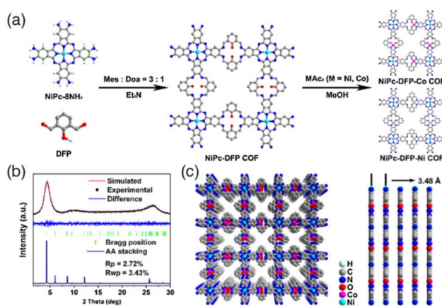
Fig. 17 (a) The syntheses route of NiPc-DFP-M COF ( M = \text{Co} and \text{Ni} ). (b) PXRD patterns of NiPc-DFP-Co COF. (c) AA stacking mode for NiPc-DFP-Co COF. Reprinted with permission from ref. 42. Copyright 2023 CCS Chem.
