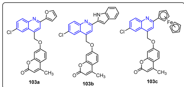
Scheme 24 YbCl 3 -catalyzed synthetic protocol for the preparation of arylmethoxy-chromen-2-one derivatives 103 .
