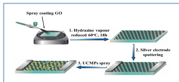
Fig. 1 Fabrication process of IR photodetector based on RGO and UCMPs.
